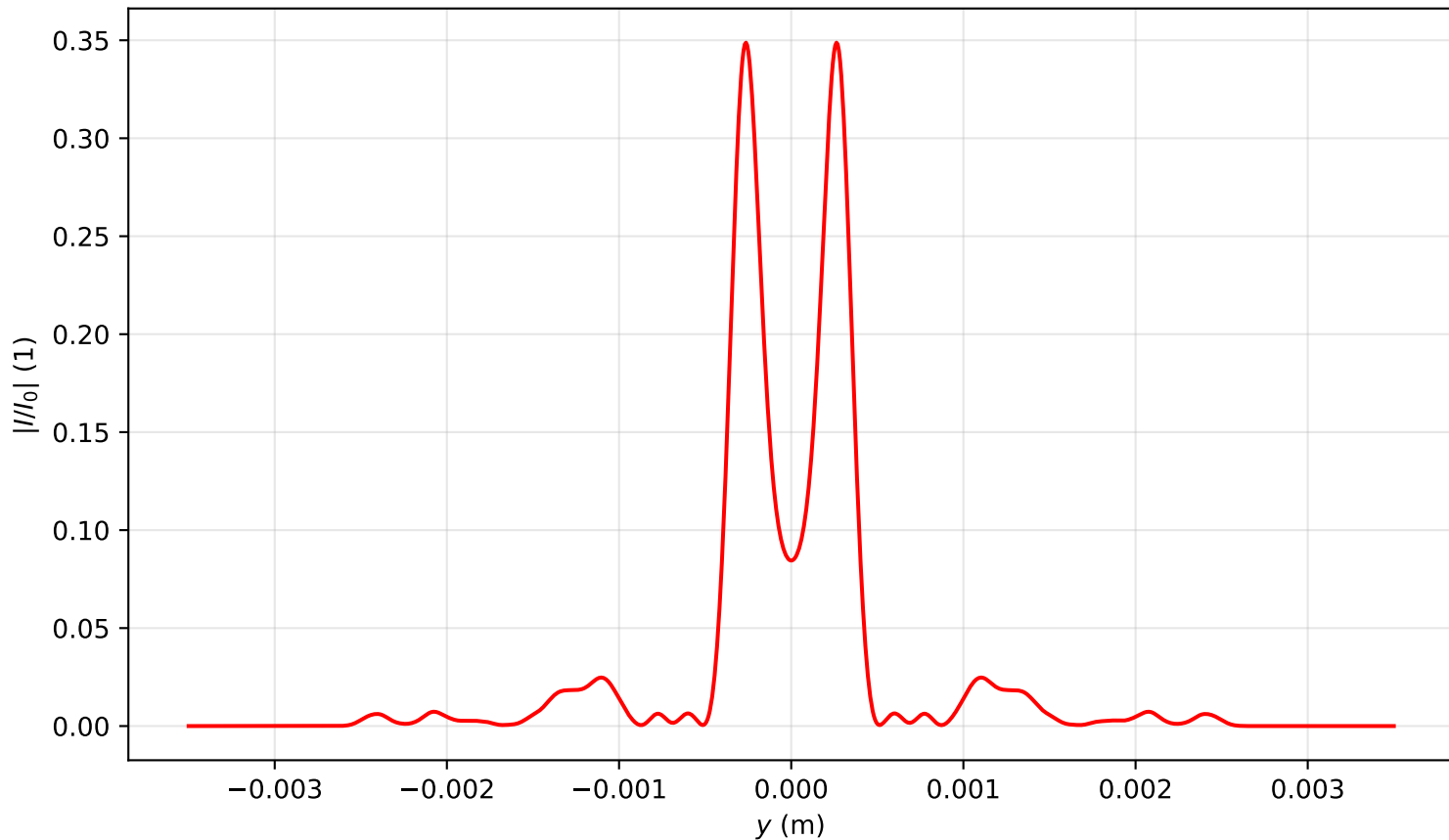
Intensity profile I(x=0, y, z=2.627)/I_0 , P_{in}=12.0P_{cr} , artificial time
