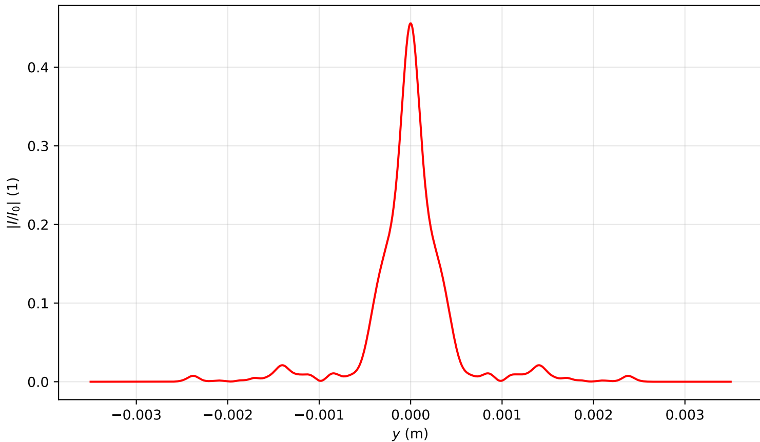
Intensity profile I(x=0, y, z=2.866)/I_0 , P_{in}=12.0P_{cr} , artificial time
