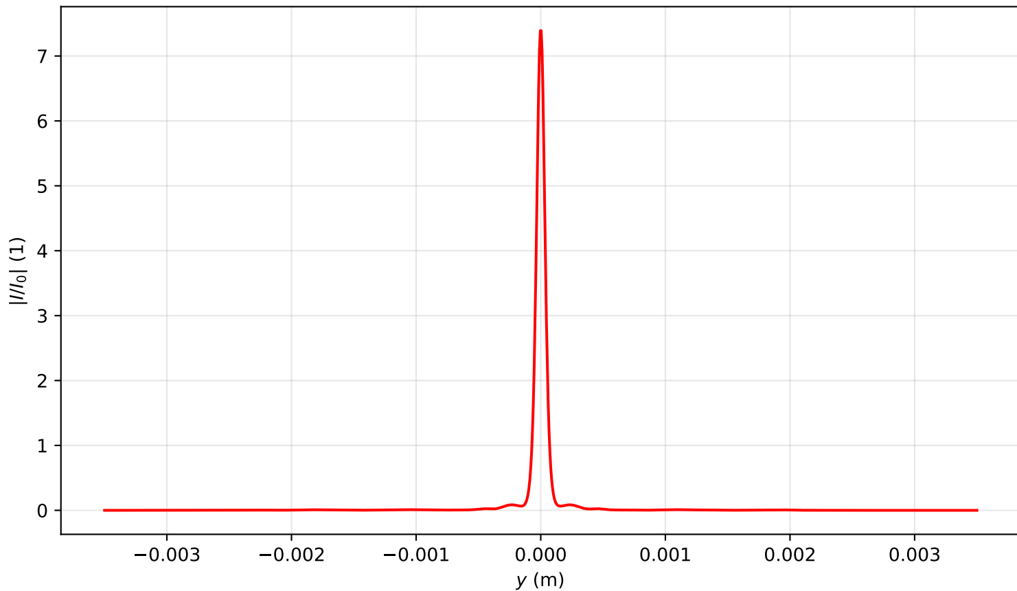
Intensity profile I(x=0, y, z=3.344)/I_0 , P_{in}=12.0P_{cr} , artificial time
