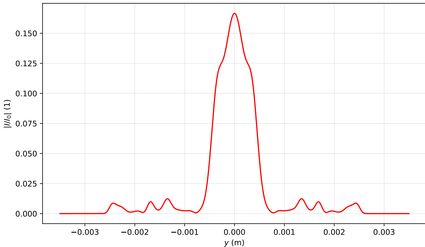
Intensity profile I(x=0, y, z=3.821)/I_0 , P_{in}=12.0\text{Pcr} , artificial time
