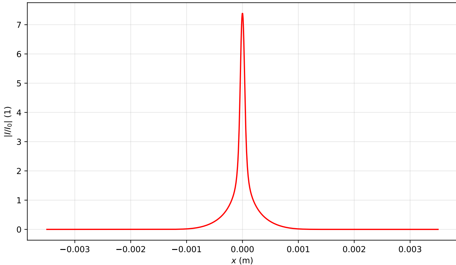
Intensity profile I(x, y = 0, z = 0.239)/I_0 , P_{in}=12.5P_{cr} , artificial time
