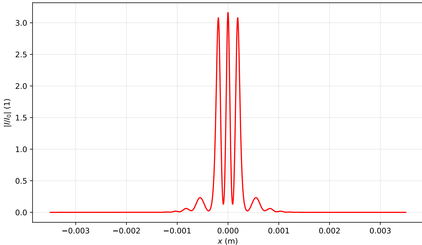
Intensity profile I(x, y = 0, z = 0.478)/I_0 , P_{in}=12.5P_{cr} , artificial time
