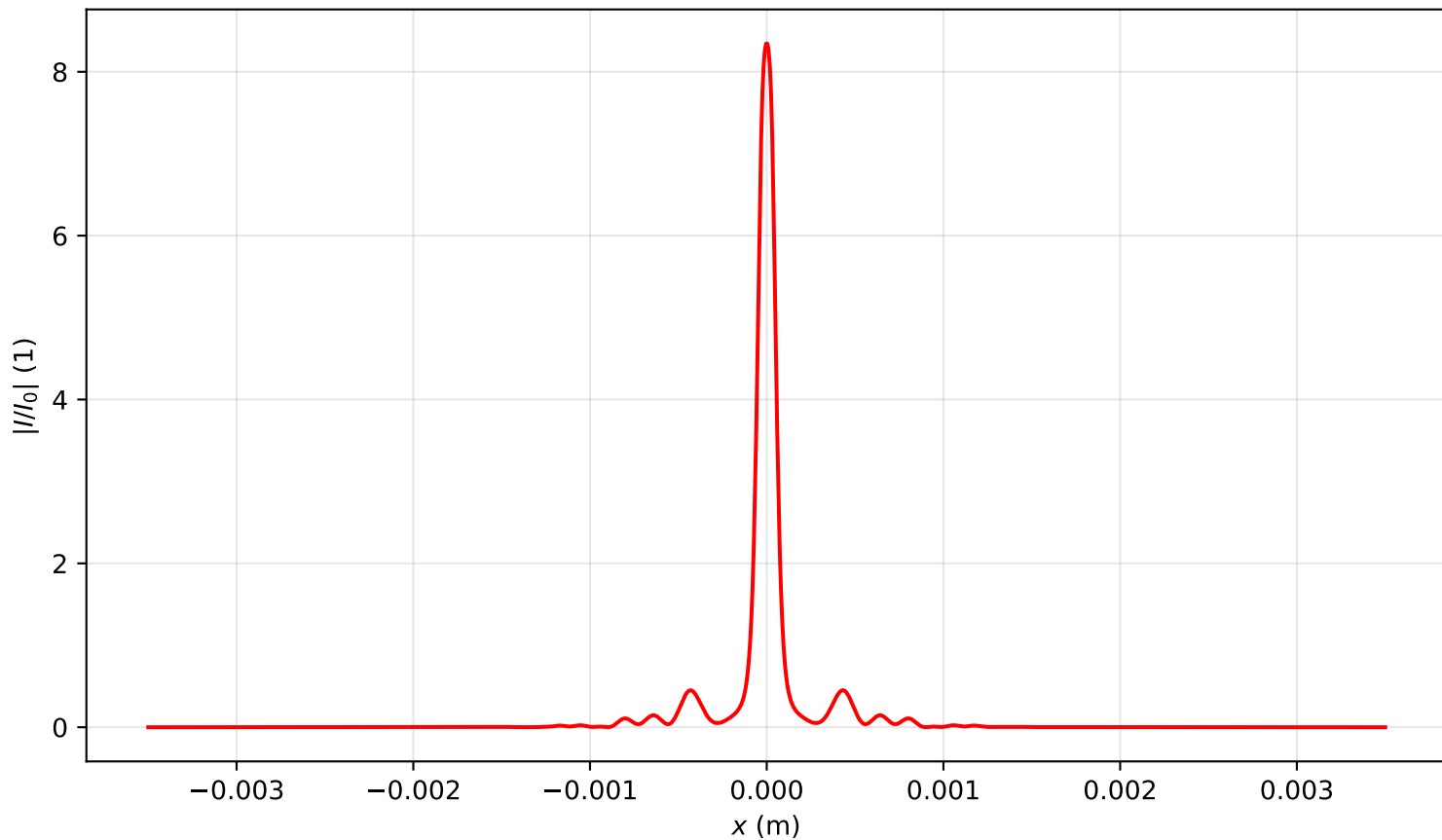
Intensity profile I(x, y = 0, z = 0.716)/I_0 , P_{in}=12.5P_{cr} , artificial time
