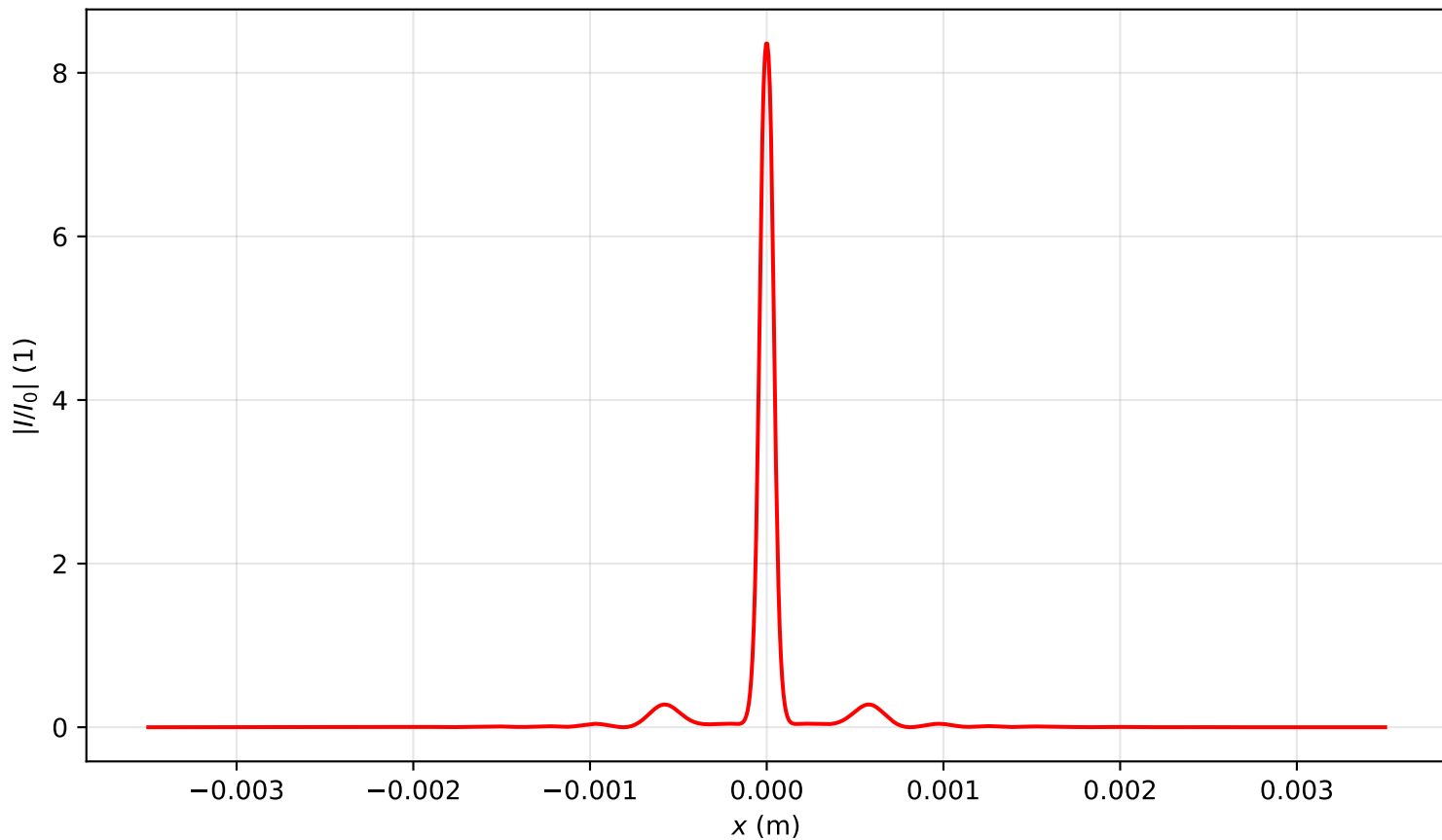
Intensity profile I(x, y = 0, z = 0.955)/I_0 , P_{in}=12.5P_{cr} , artificial time
