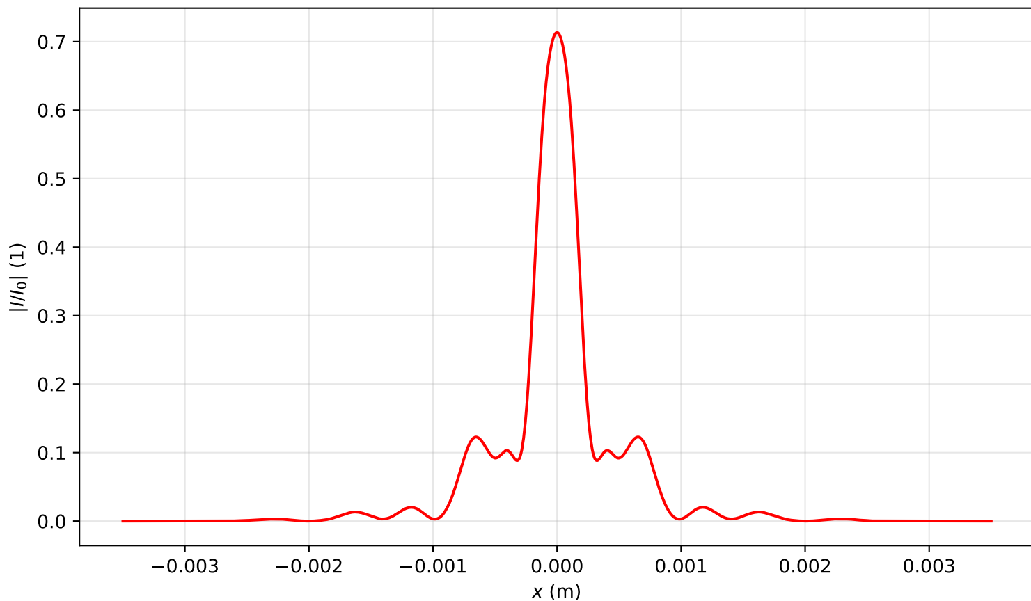
Intensity profile I(x, y = 0, z = 1.194)/I_0 , P_{in}=12.5P_{cr} , artificial time
