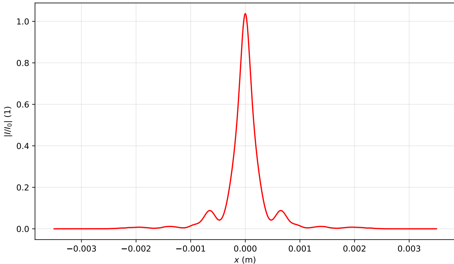
Intensity profile I(x, y = 0, z = 1.433)/I_0 , P_{in}=12.5P_{cr} , artificial time
