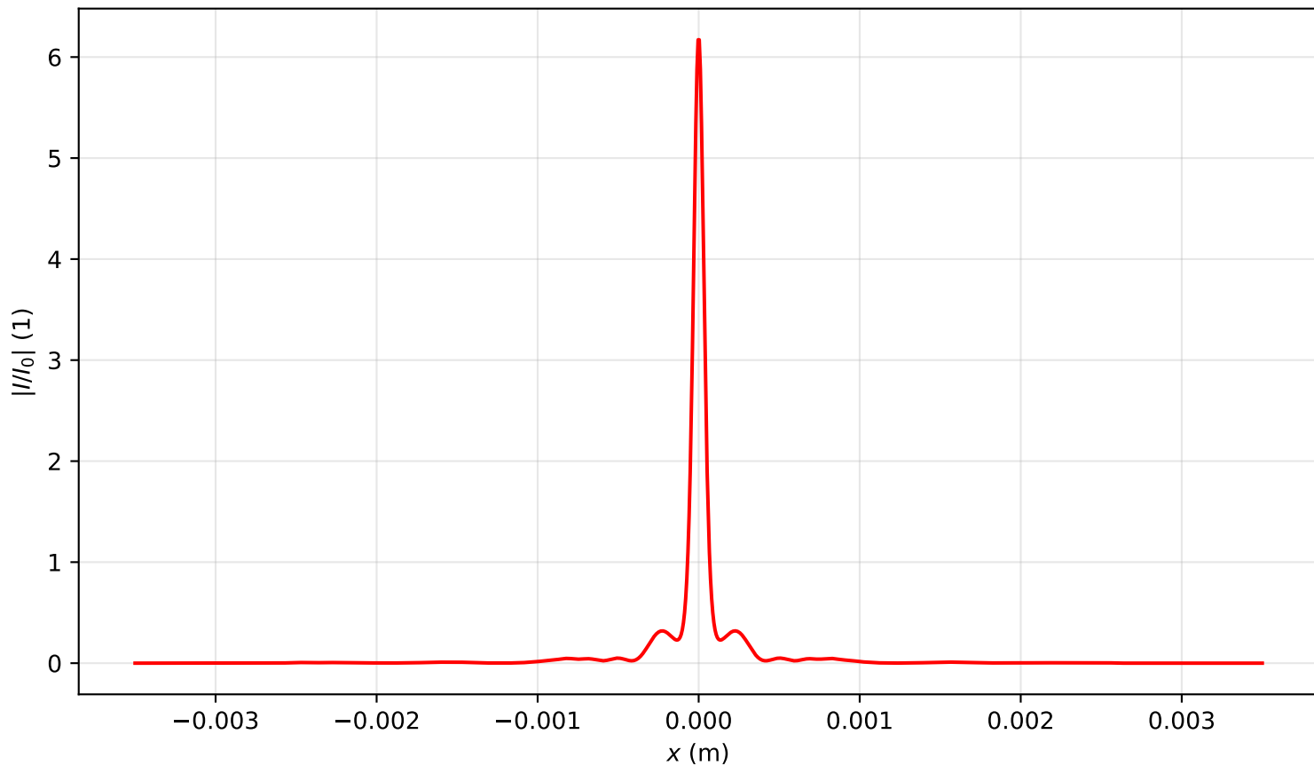
Intensity profile I(x, y = 0, z = 1.672)/I_0 , P_{in}=12.5P_{cr} , artificial time
