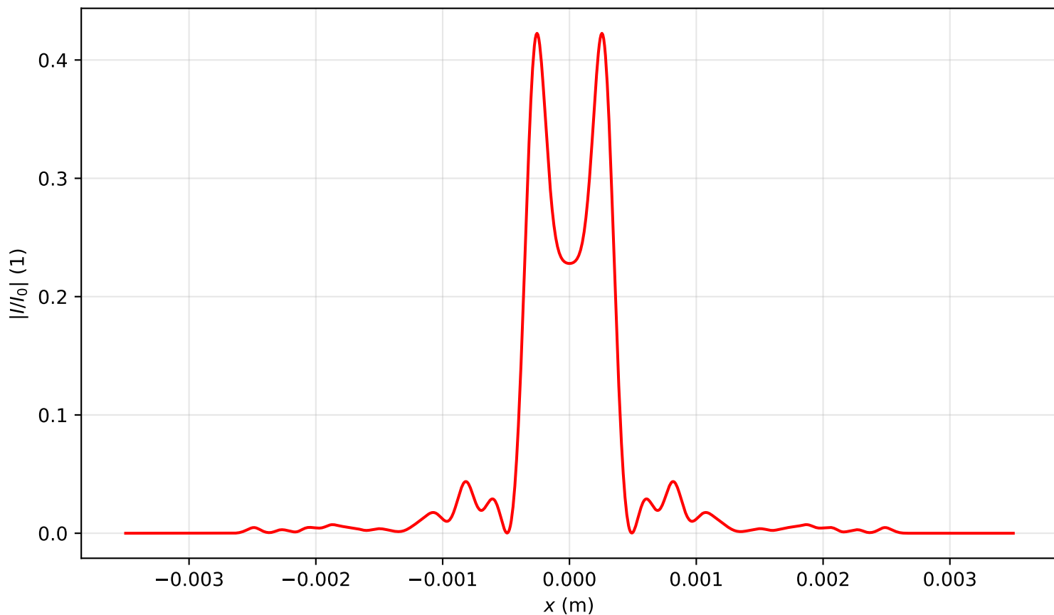
Intensity profile I(x, y = 0, z = 1.911)/I_0 , P_{in}=12.5P_{cr} , artificial time
