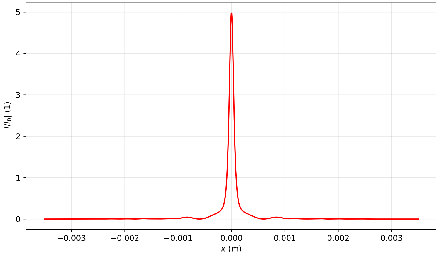
Intensity profile I(x, y = 0, z = 2.149)/I_0 , P_{in}=12.5P_{cr} , artificial time
