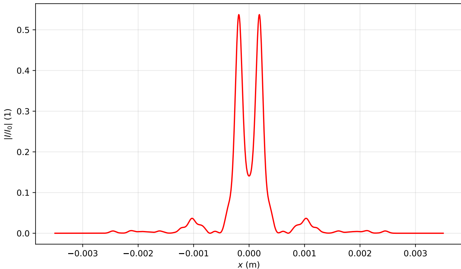
Intensity profile I(x, y = 0, z = 2.388)/I_0 , P_{in}=12.5P_{cr} , artificial time
