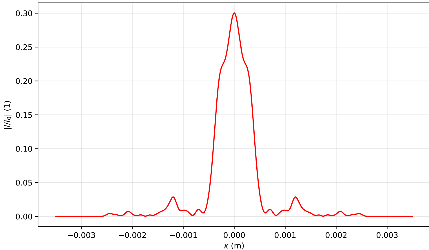
Intensity profile I(x, y = 0, z = 2.627)/I_0 , P_{in}=12.5P_{cr} , artificial time
