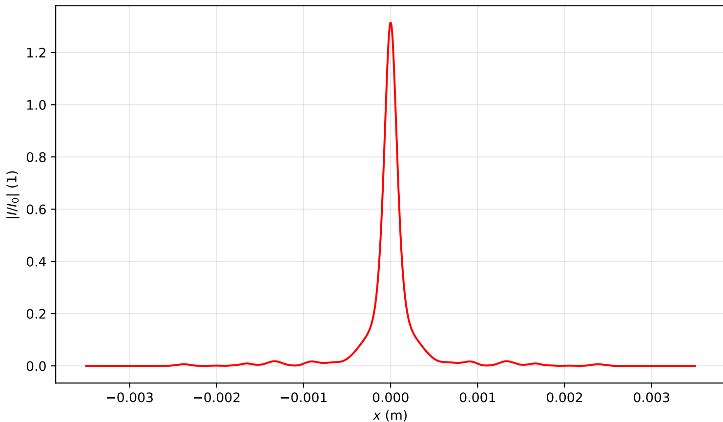
Intensity profile I(x, y = 0, z = 2.866)/I_0 , P_{in}=12.5P_{cr} , artificial time
