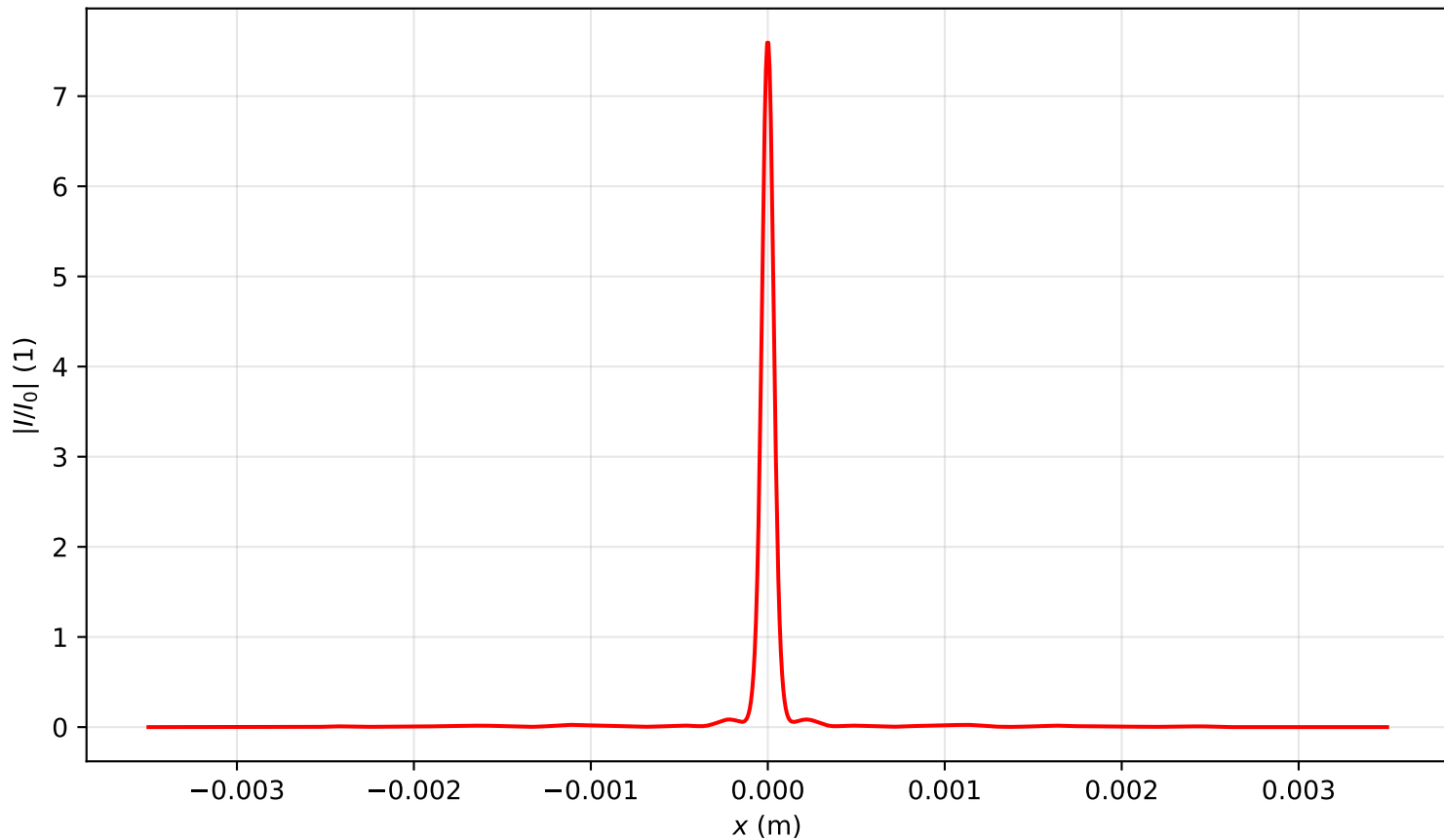
Intensity profile I(x, y = 0, z = 3.105)/I_0 , P_{in}=12.5P_{cr} , artificial time
