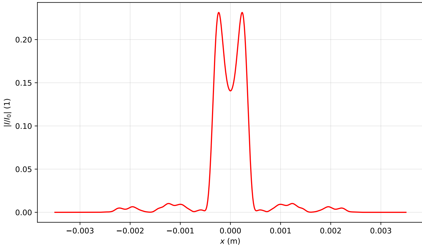
Intensity profile I(x, y = 0, z = 3.344)/I_0 , P_{in}=12.5P_{cr} , artificial time
