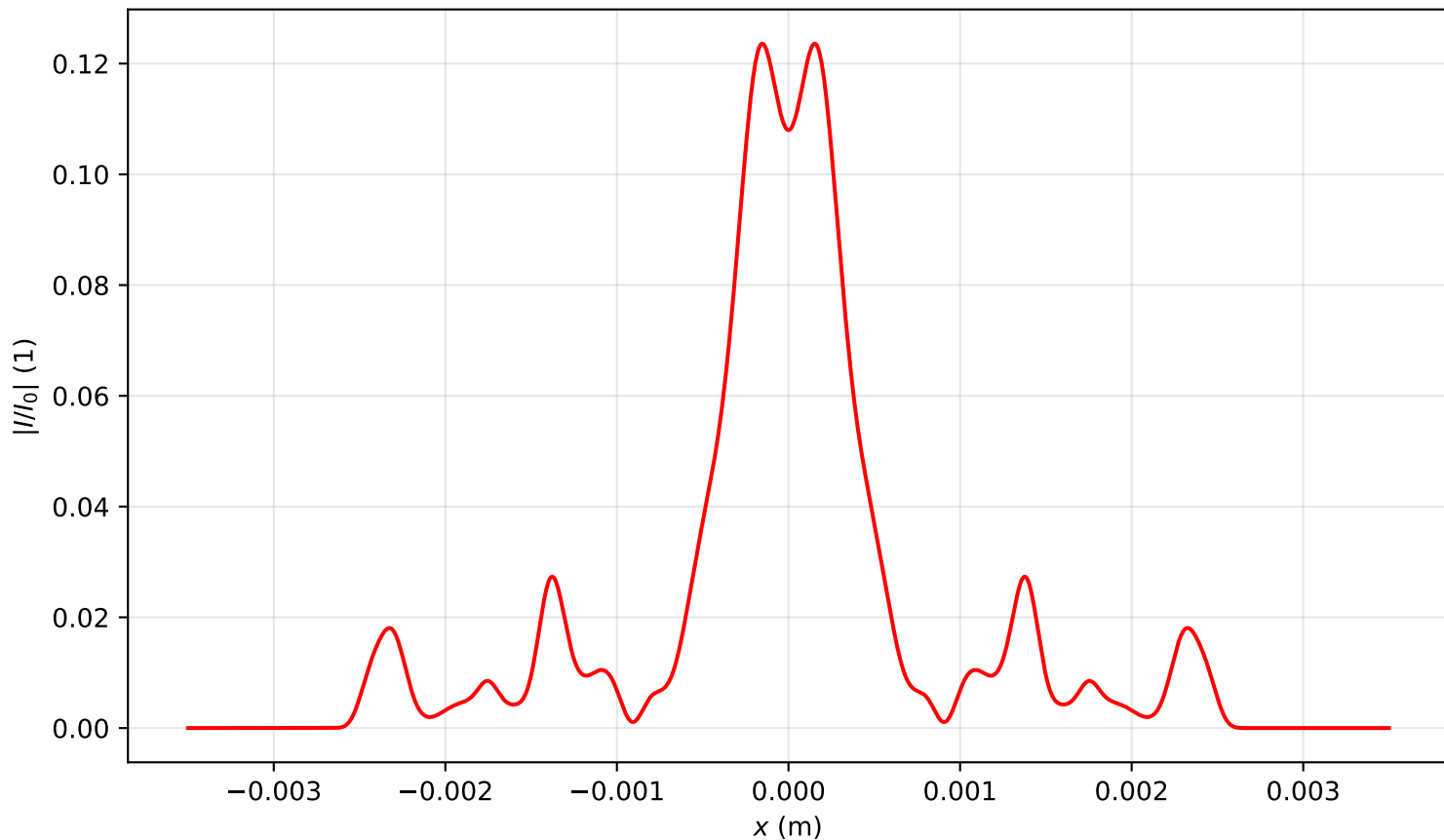
Intensity profile I(x, y = 0, z = 3.582)/I_0 , P_{in}=12.5P_{cr} , artificial time
