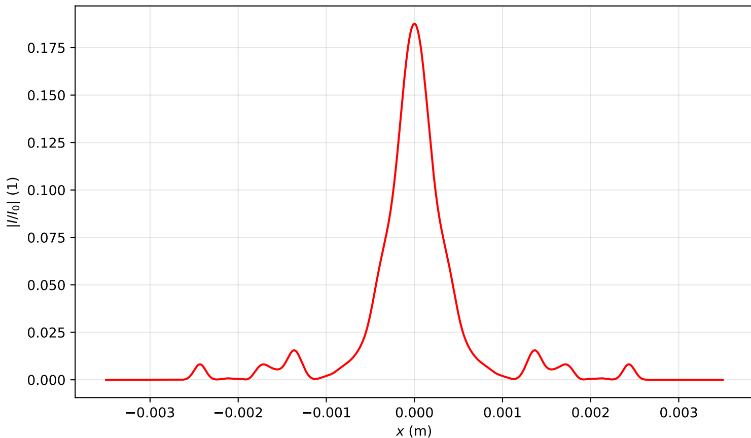
Intensity profile I(x, y = 0, z = 3.821)/I_0 , P_{in}=12.5\text{Pcr} , artificial time
