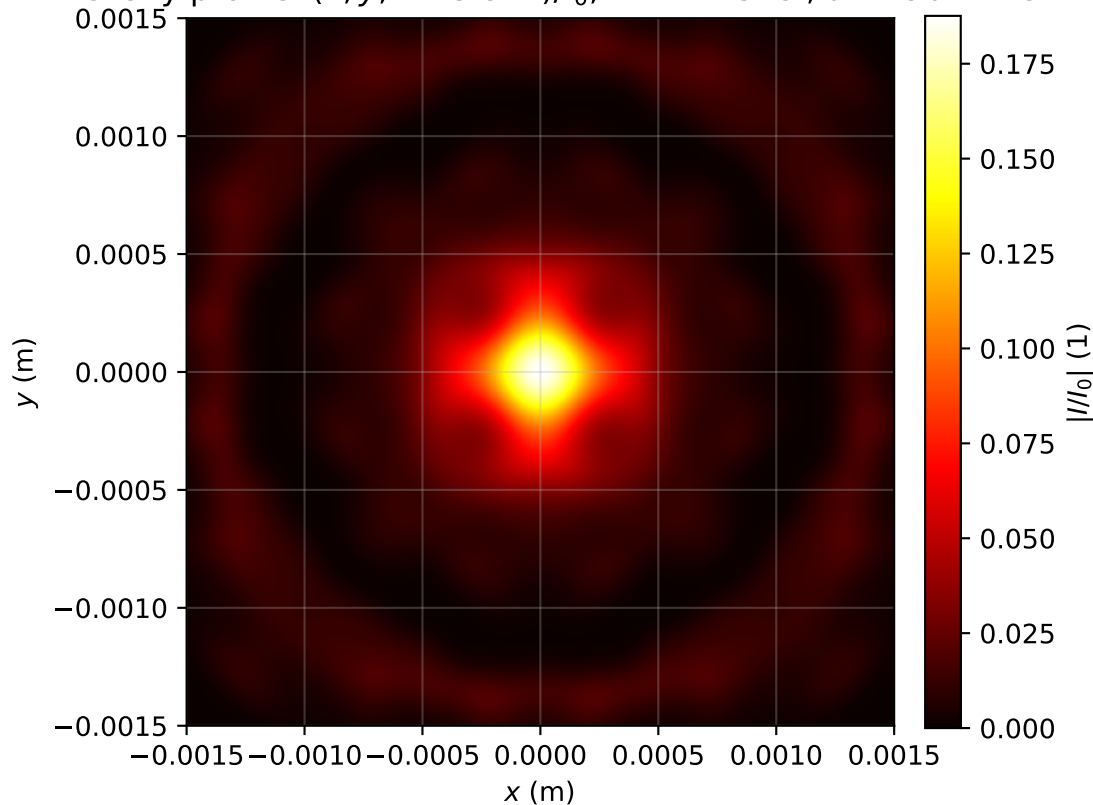
Intensity profile I(x, y, z = 3.821)/I_0 , P_{in}=12.5P_{cr} , artificial time
