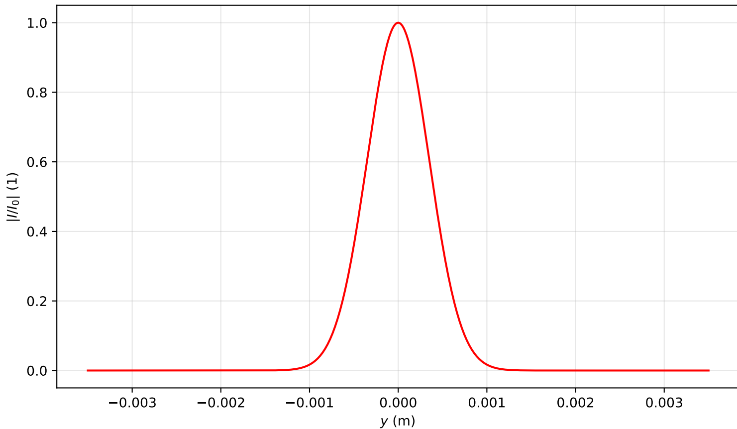
Intensity profile I(x=0, y, z=0.000)/I_0 , P_{in}=12.5P_{cr} , artificial time
