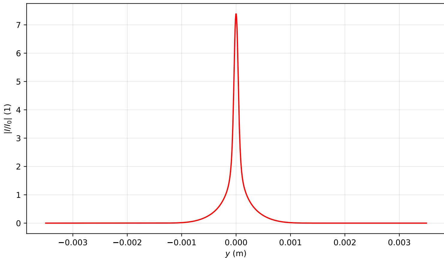
Intensity profile I(x=0, y, z=0.239)/I_0 , P_{in}=12.5P_{cr} , artificial time
