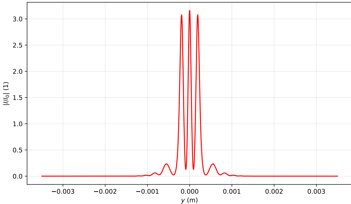
Intensity profile I(x=0, y, z=0.478)/I_0 , P_{in}=12.5P_{cr} , artificial time
