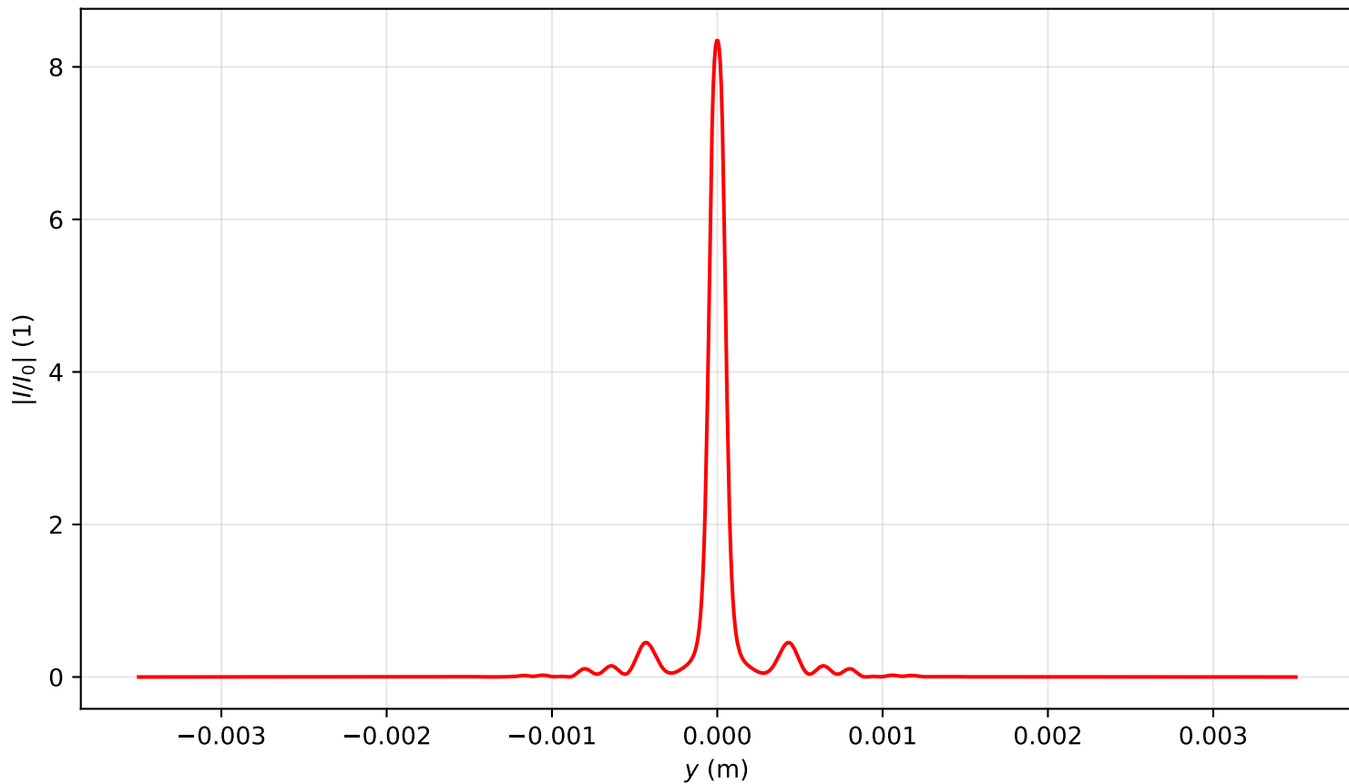
Intensity profile I(x=0, y, z=0.716)/I_0 , P_{in}=12.5P_{cr} , artificial time
