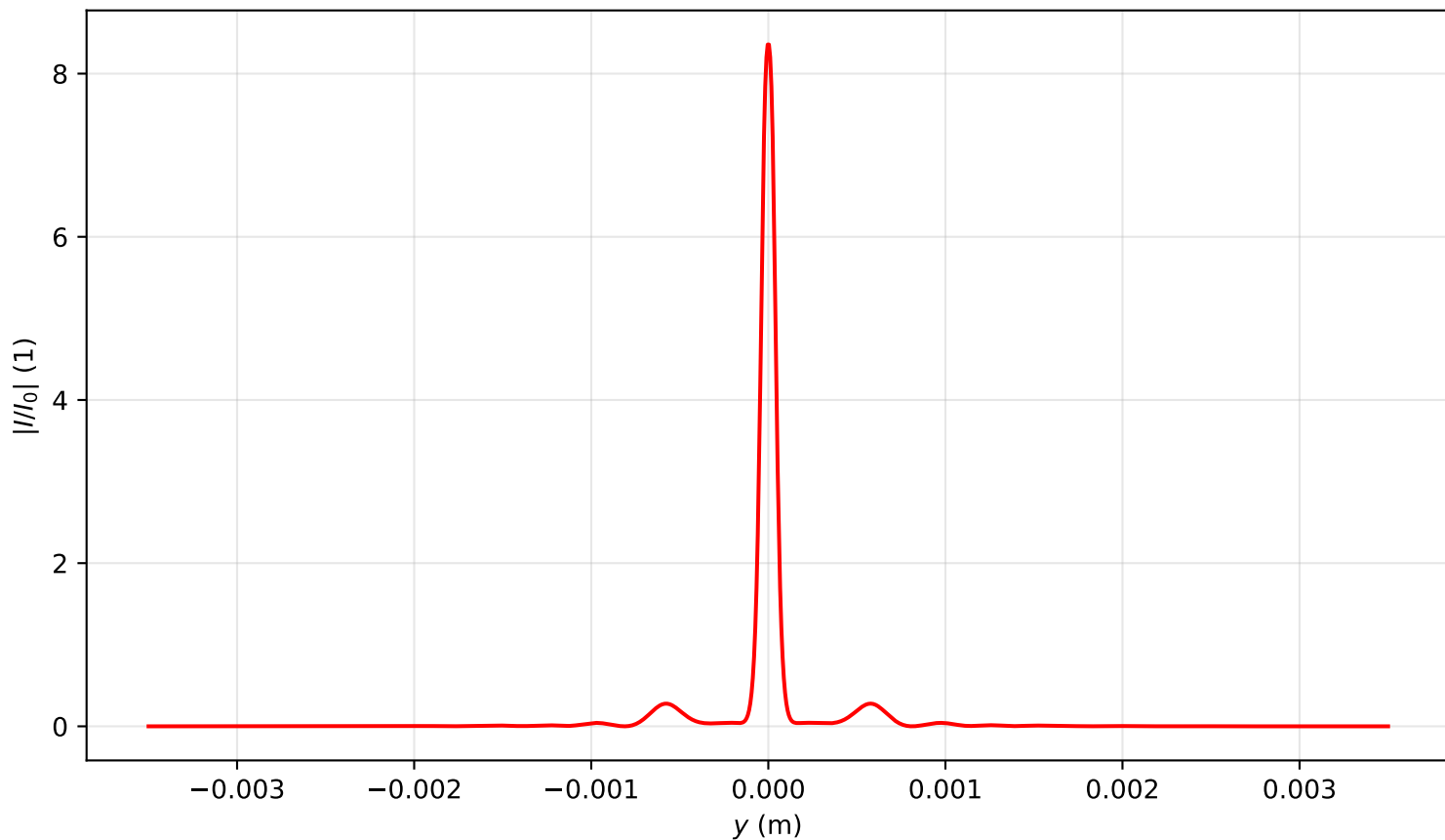
Intensity profile I(x=0, y, z=0.955)/I_0 , P_{in}=12.5P_{cr} , artificial time
