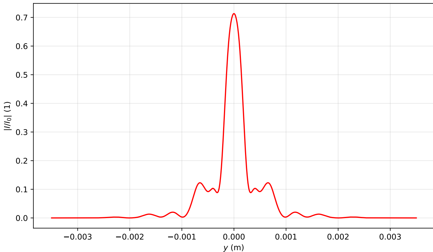
Intensity profile I(x=0, y, z=1.194)/I_0 , P_{in}=12.5P_{cr} , artificial time
