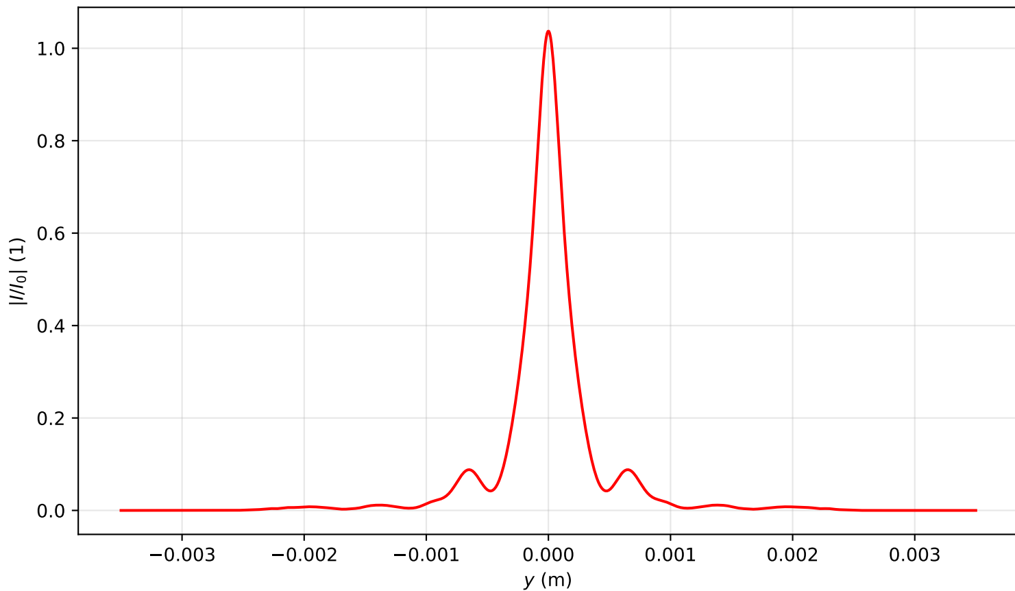
Intensity profile I(x=0, y, z=1.433)/I_0 , P_{in}=12.5P_{cr} , artificial time
