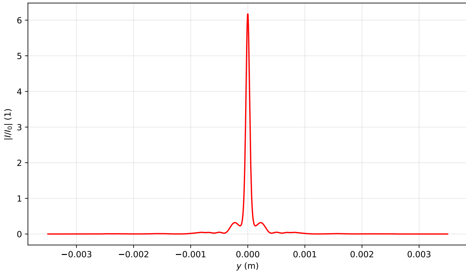
Intensity profile I(x=0, y, z=1.672)/I_0 , P_{in}=12.5P_{cr} , artificial time
