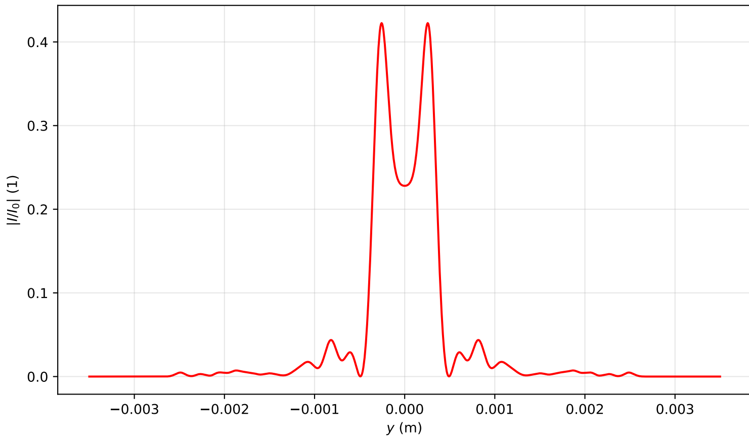
Intensity profile I(x=0, y, z=1.911)/I_0 , P_{in}=12.5P_{cr} , artificial time
