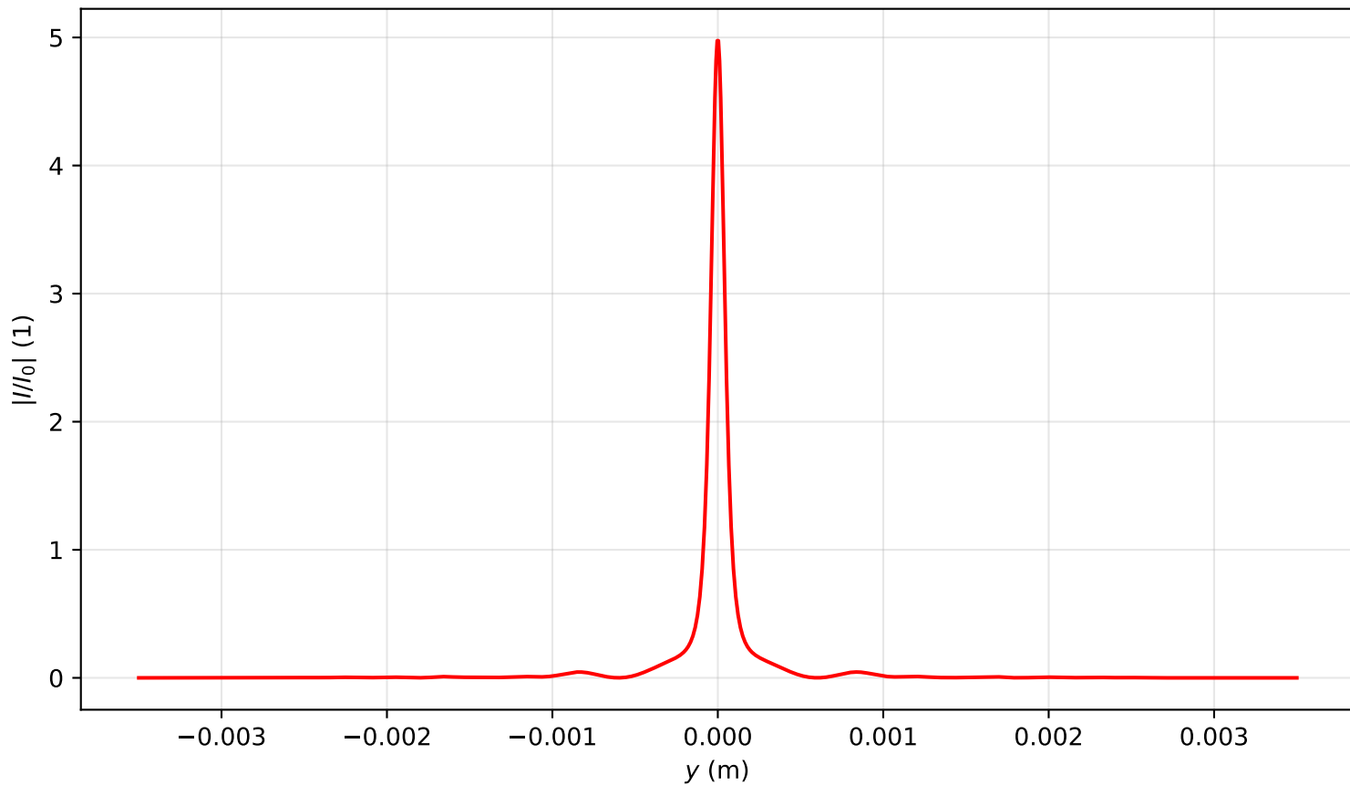
Intensity profile I(x=0, y, z=2.149)/I_0 , P_{in}=12.5P_{cr} , artificial time
