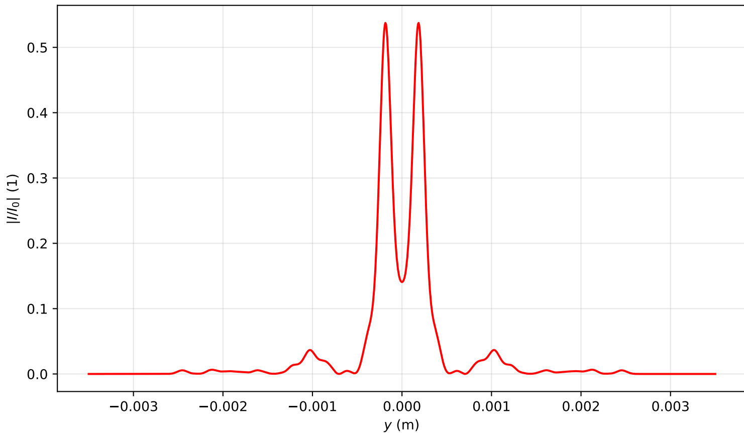
Intensity profile I(x=0, y, z=2.388)/I_0 , P_{in}=12.5P_{cr} , artificial time
