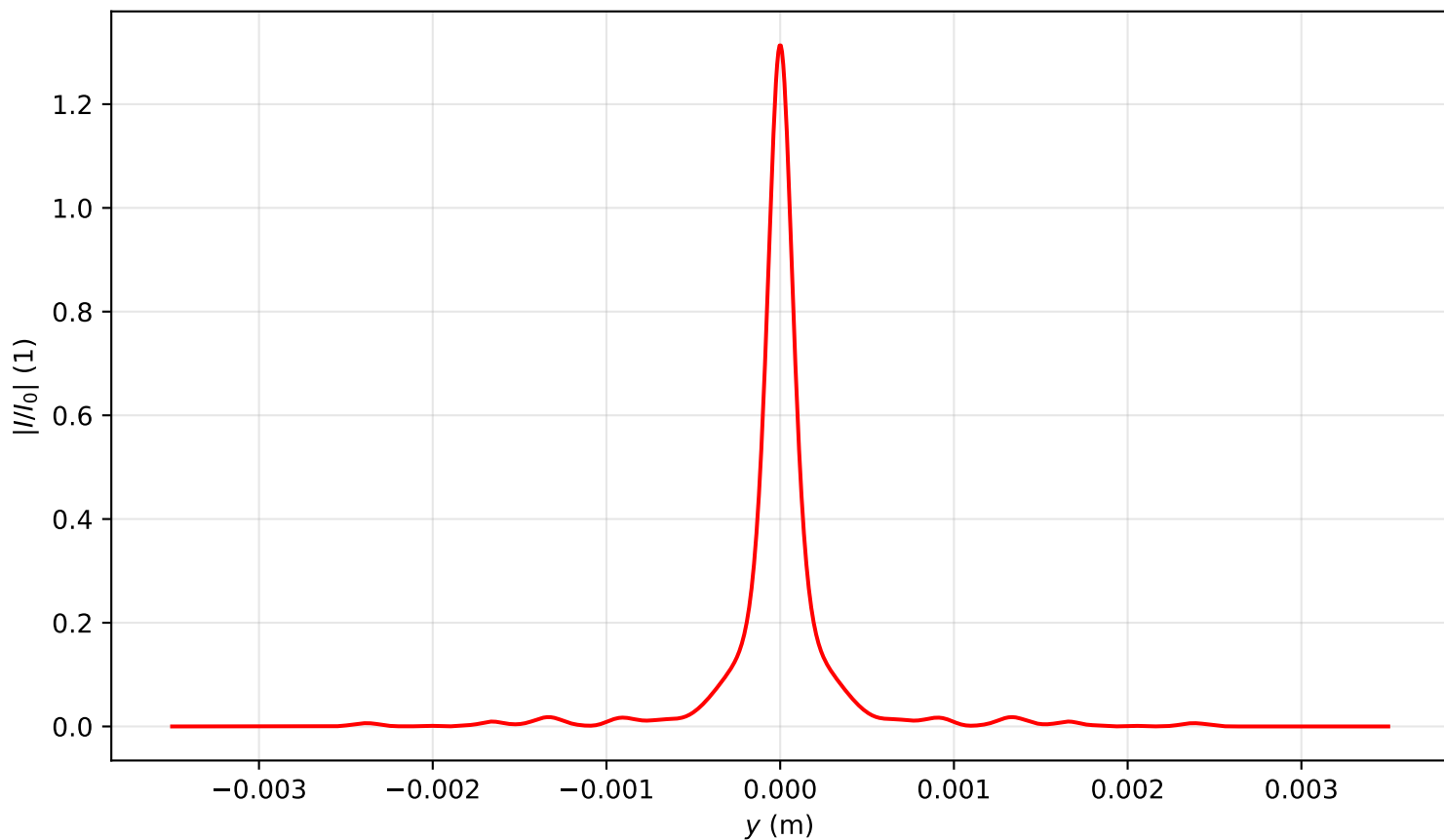
Intensity profile I(x=0, y, z=2.866)/I_0 , P_{in}=12.5P_{cr} , artificial time
