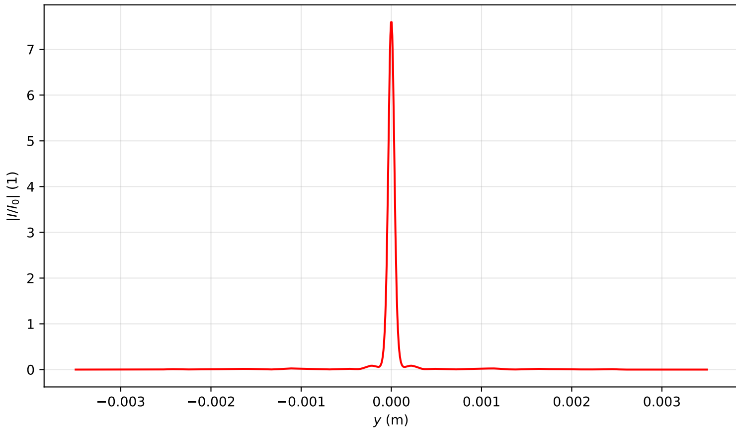
Intensity profile I(x=0, y, z=3.105)/I_0 , P_{in}=12.5P_{cr} , artificial time
