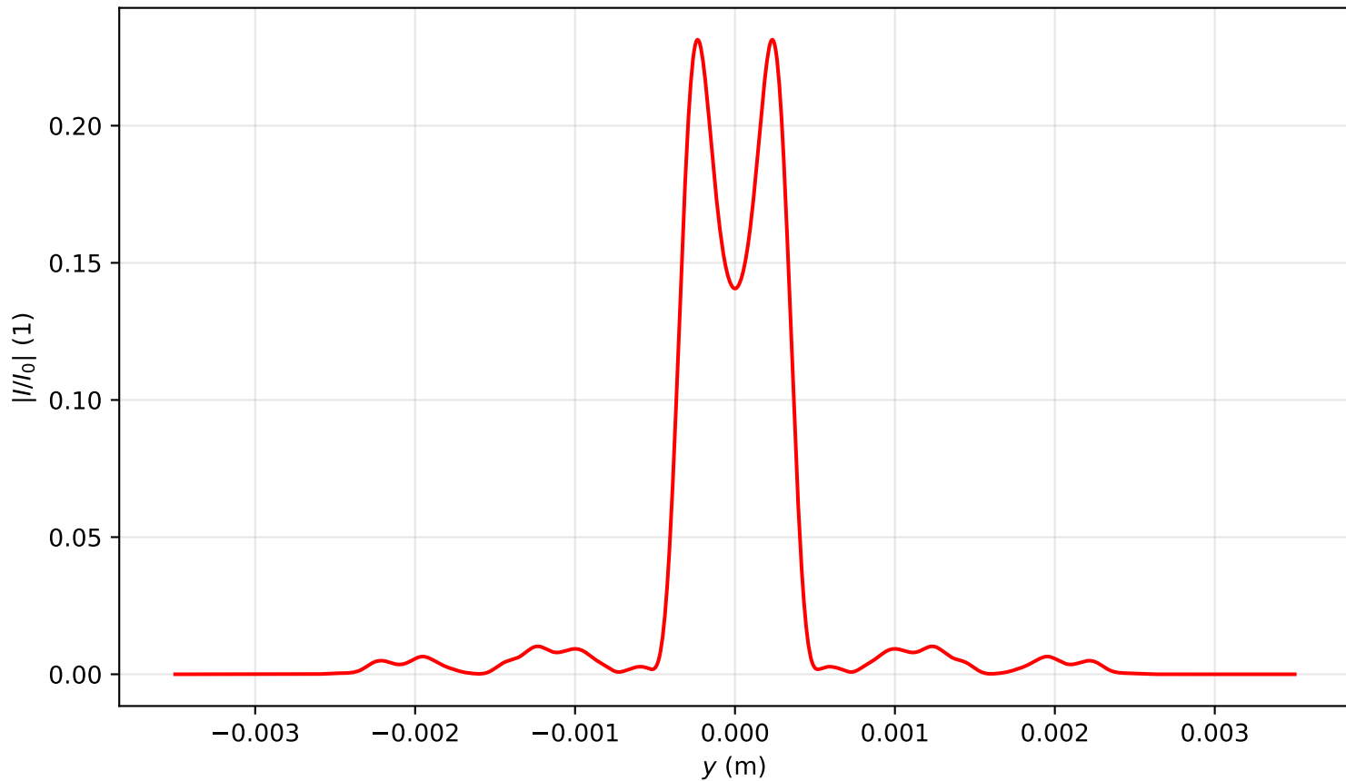
Intensity profile I(x=0, y, z=3.344)/I_0 , P_{in}=12.5P_{cr} , artificial time
