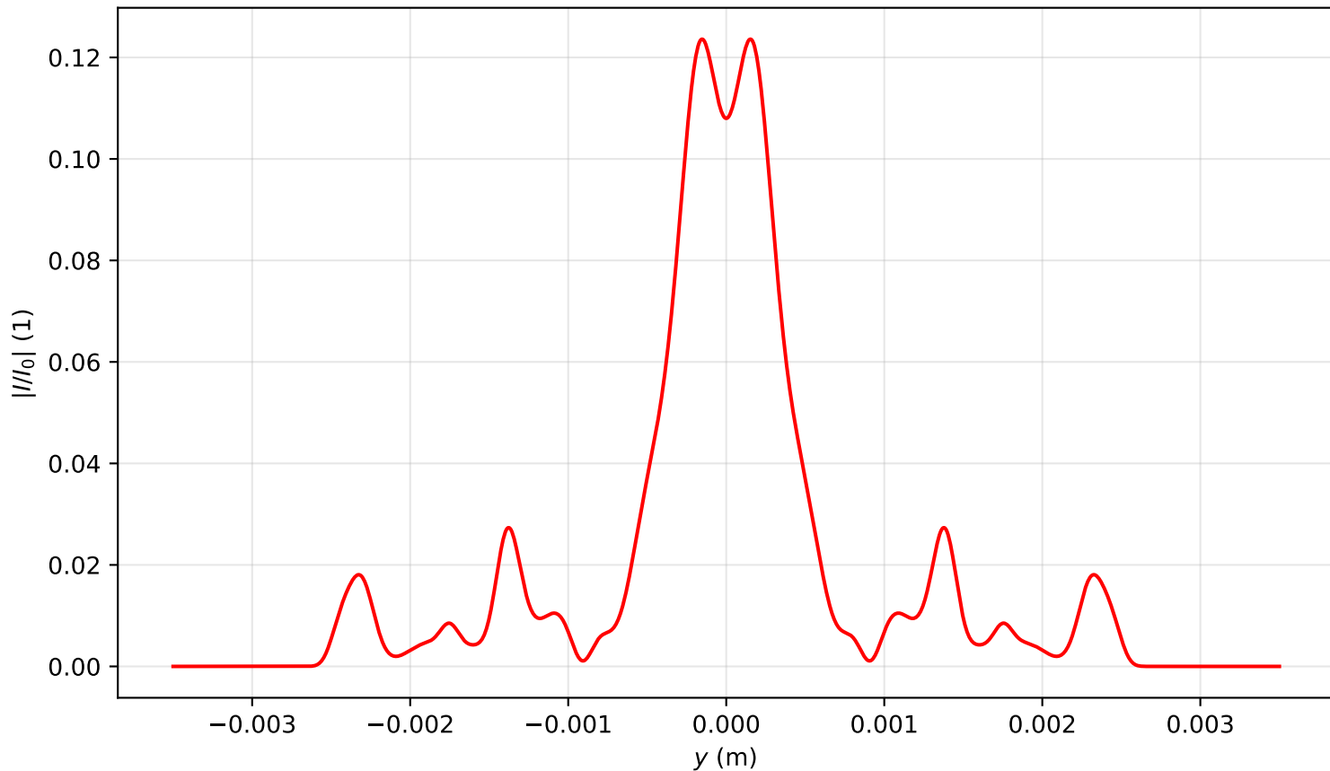
Intensity profile I(x = 0, y, z = 3.582)/I_0 , P_{in}=12.5P_{cr} , artificial time
