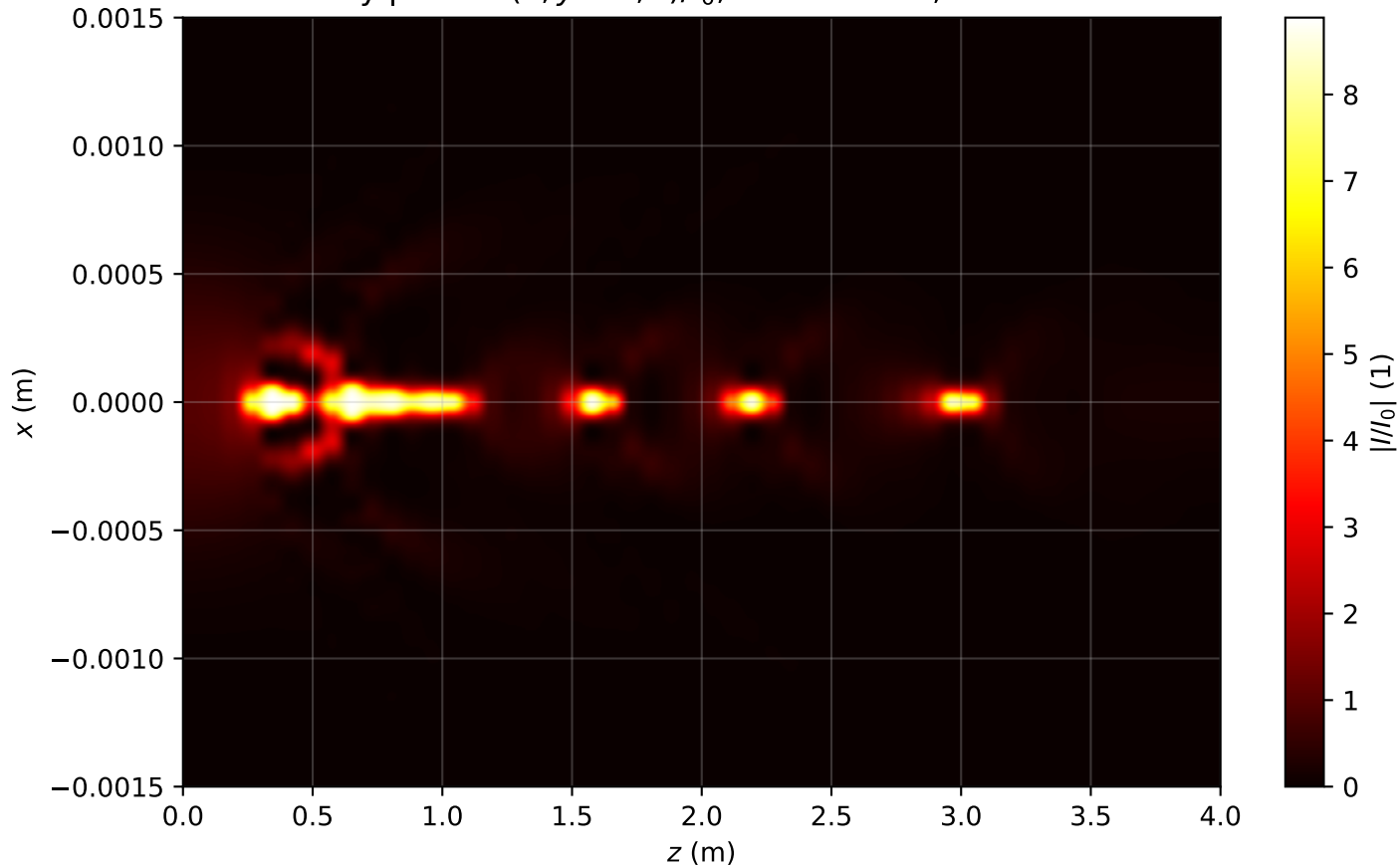
Intensity profile I(x, y = 0, z)/I_0 , P_{in}=12.5\text{Pcr} , artificial time
