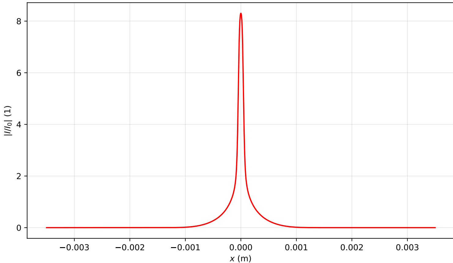
Intensity profile I(x, y = 0, z = 0.239)/I_0 , P_{in}=13.0P_{cr} , artificial time
