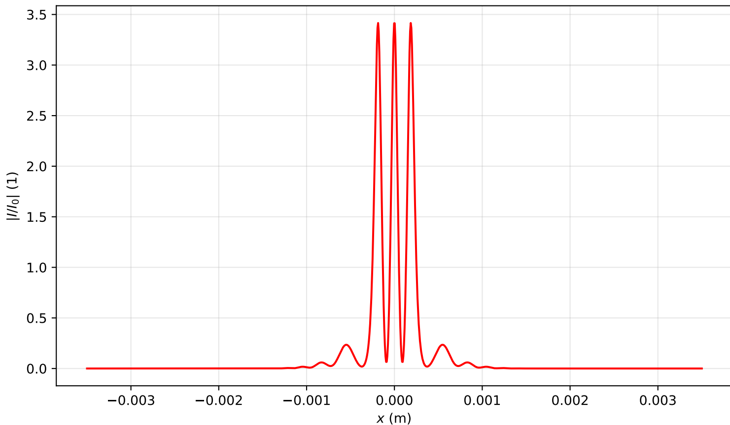
Intensity profile I(x, y = 0, z = 0.478)/I_0 , P_{in}=13.0P_{cr} , artificial time
