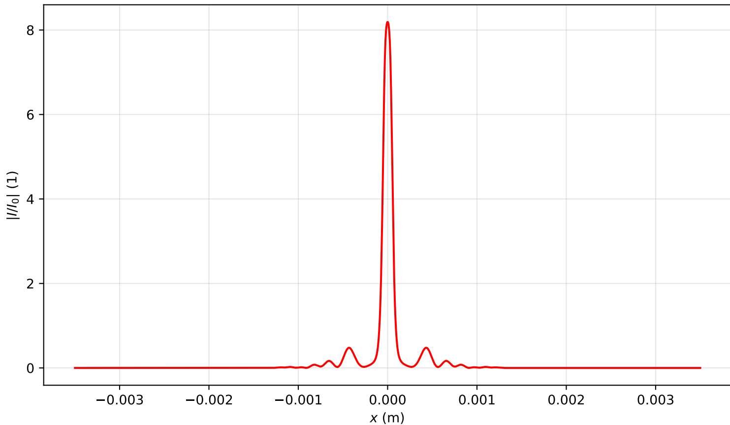
Intensity profile I(x, y = 0, z = 0.716)/I_0 , P_{in}=13.0P_{cr} , artificial time
