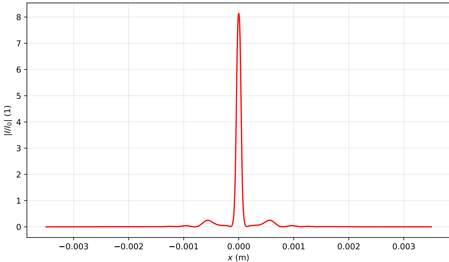
Intensity profile I(x, y = 0, z = 0.955)/I_0 , P_{in}=13.0\text{Pcr} , artificial time
