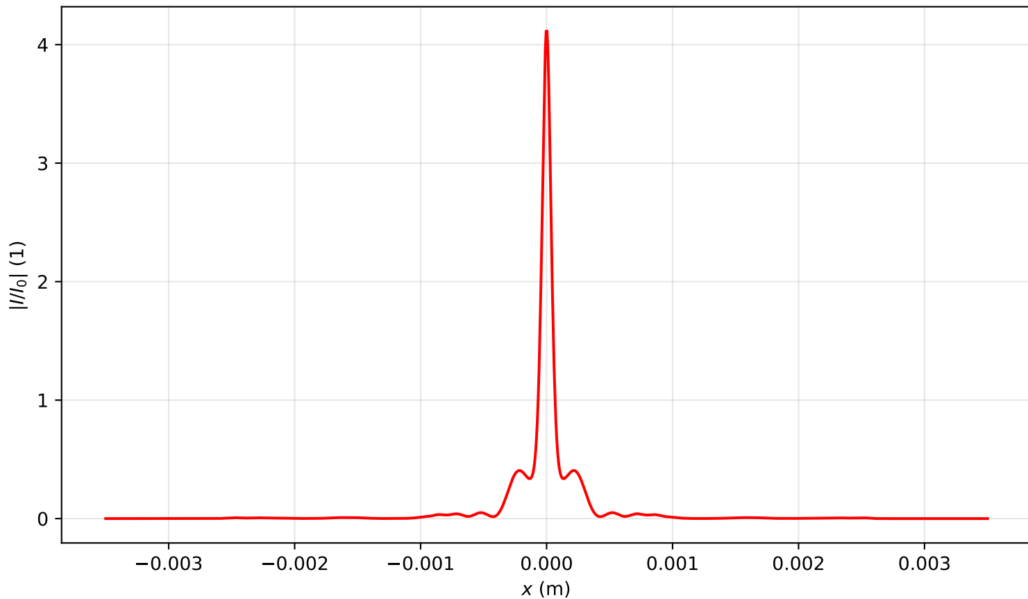
Intensity profile I(x, y = 0, z = 1.672)/I_0 , P_{in}=13.0P_{cr} , artificial time
