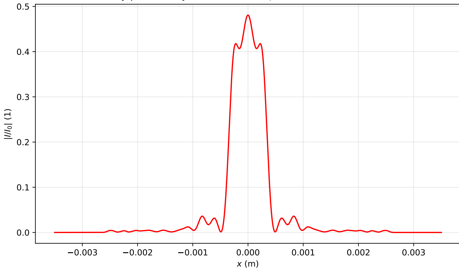
Intensity profile I(x, y = 0, z = 1.911)/I_0 , P_{in}=13.0P_{cr} , artificial time
