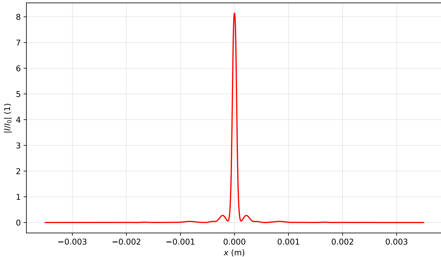
Intensity profile I(x, y = 0, z = 2.149)/I_0 , \text{Pin}=13.0\text{Pcr} , artificial time
