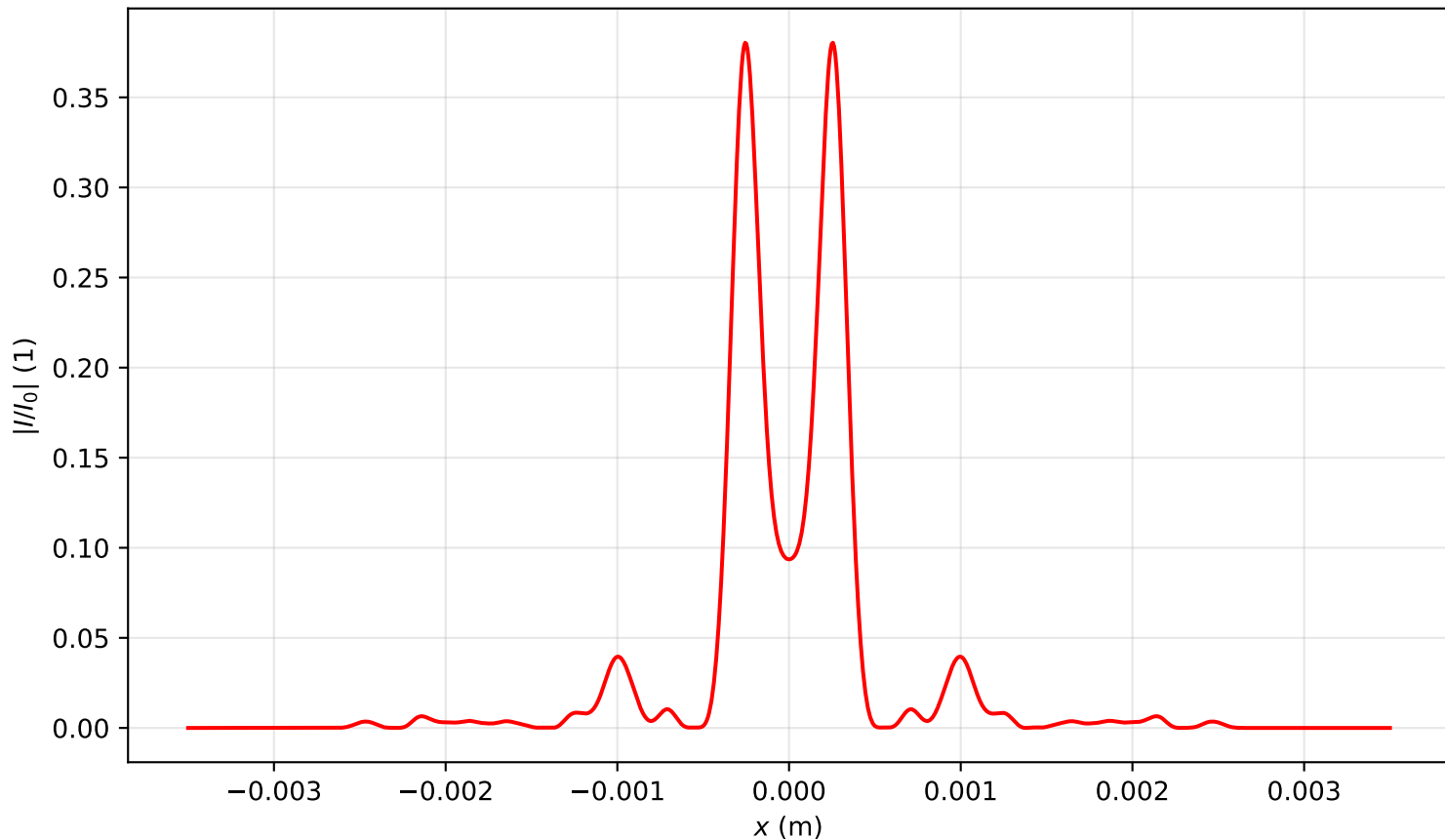
Intensity profile I(x, y = 0, z = 2.388)/I_0 , P_{in}=13.0P_{cr} , artificial time
