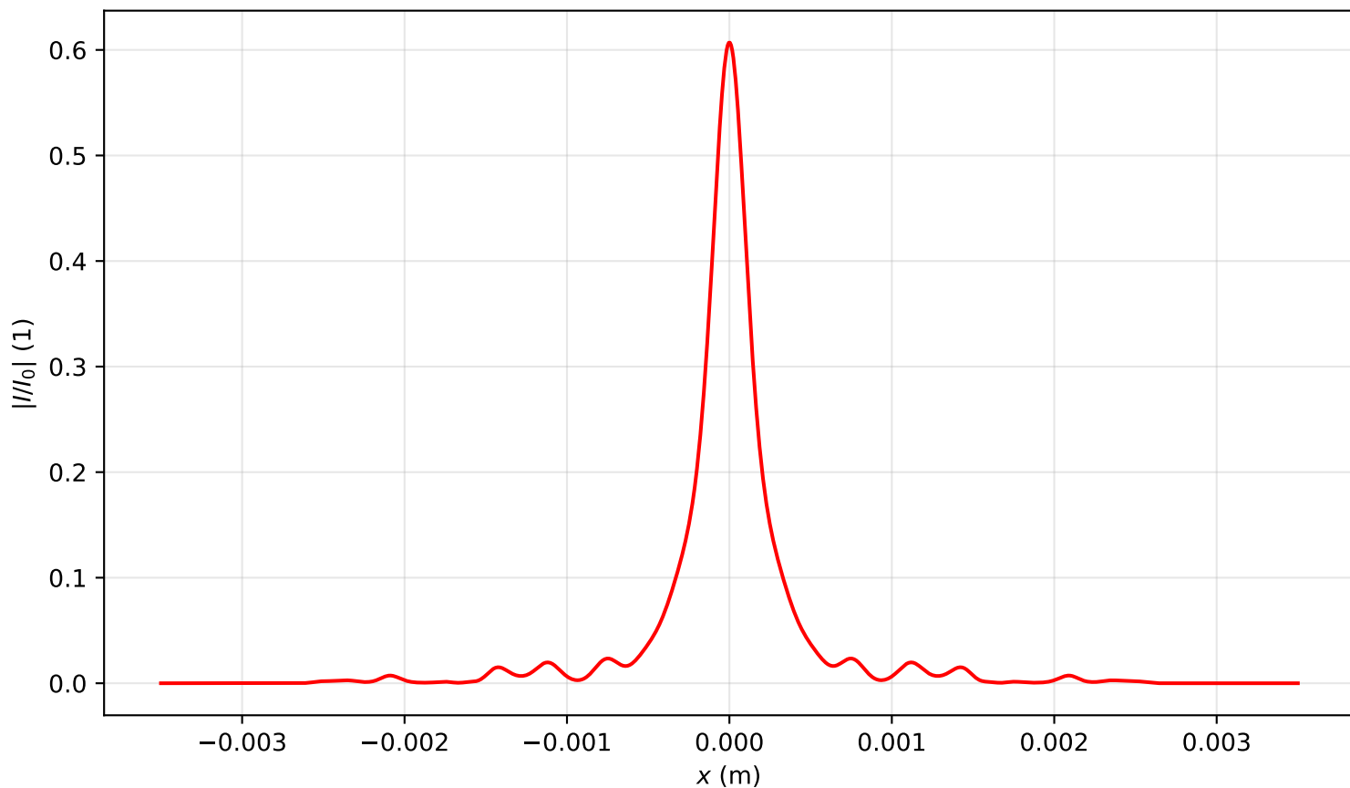
Intensity profile I(x, y = 0, z = 2.627)/I_0 , P_{in}=13.0P_{cr} , artificial time
