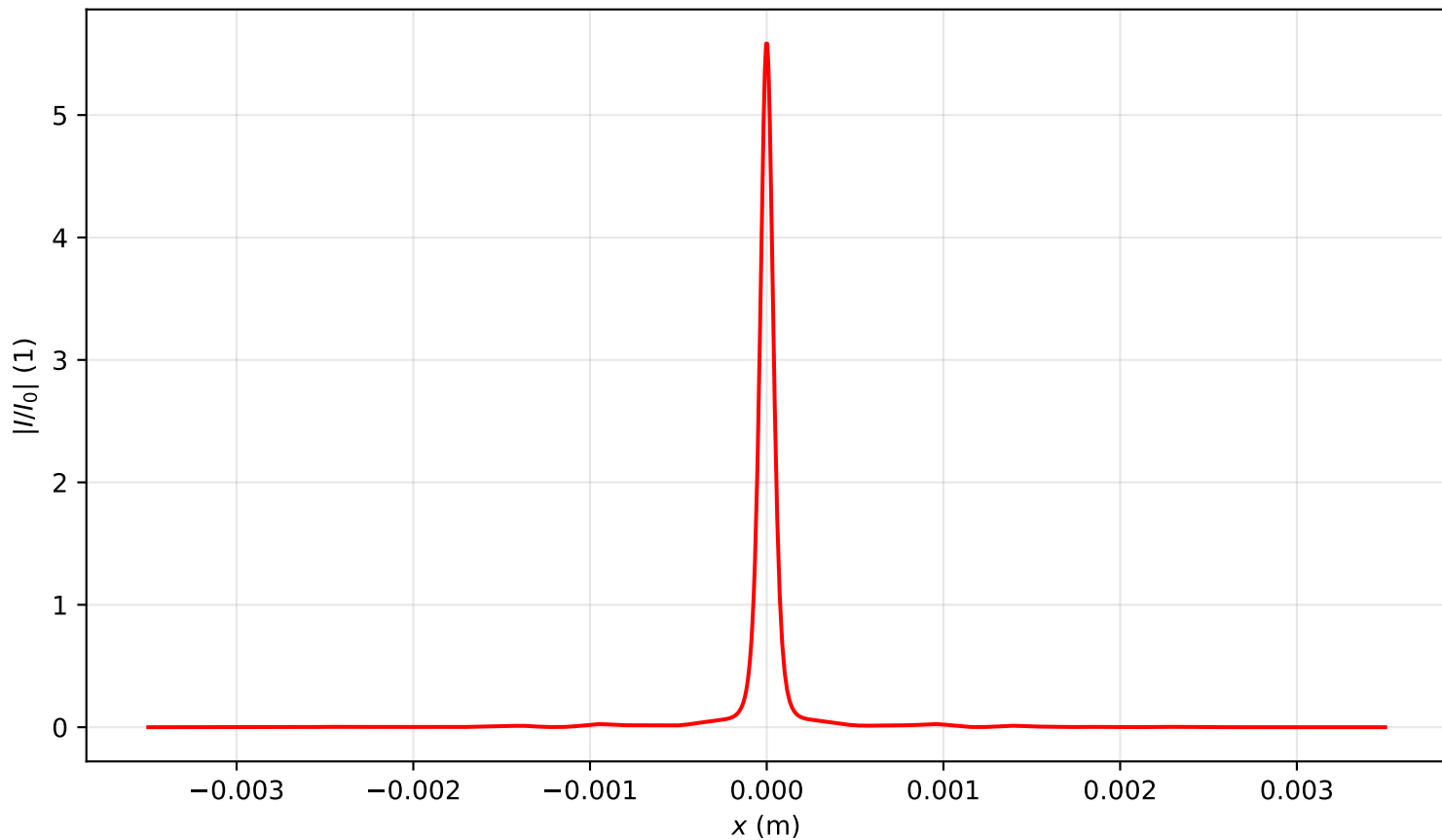
Intensity profile I(x, y = 0, z = 2.866)/I_0 , P_{in}=13.0P_{cr} , artificial time
