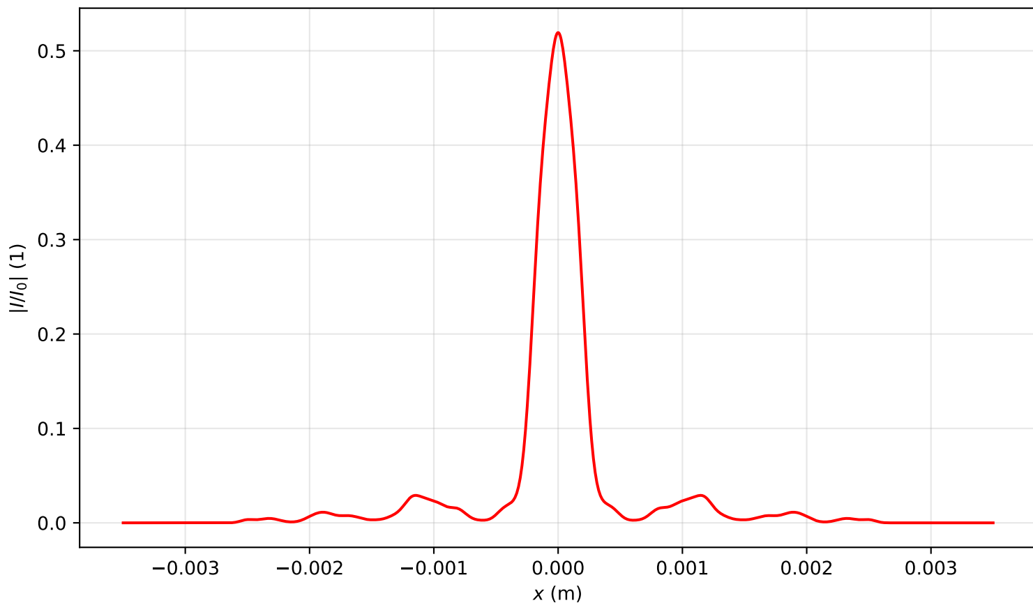
Intensity profile I(x, y = 0, z = 3.105)/I_0 , P_{in}=13.0P_{cr} , artificial time
