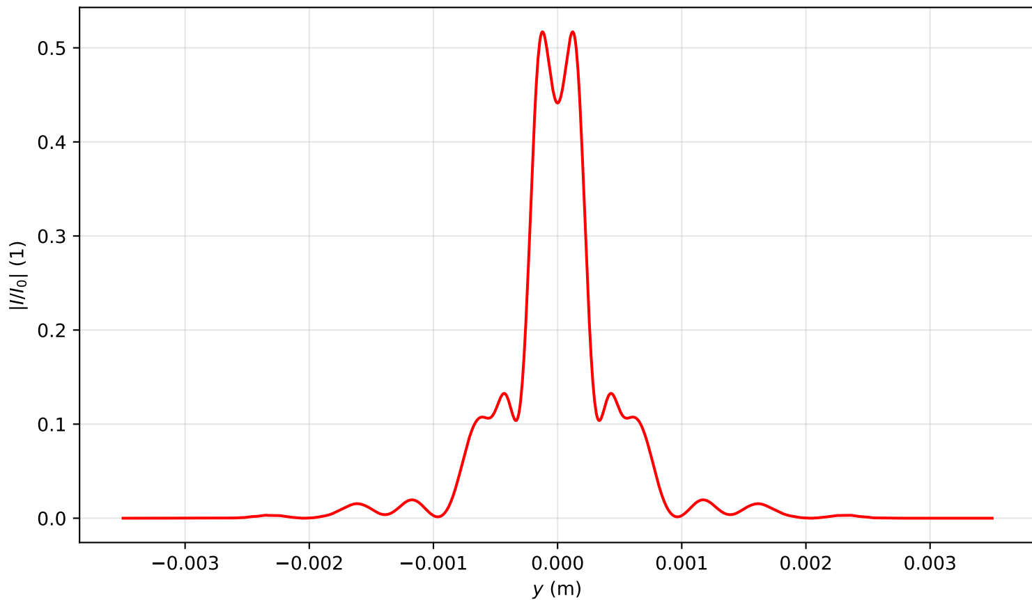
Intensity profile I(x=0, y, z=1.194)/I_0 , P_{in}=13.0P_{cr} , artificial time
