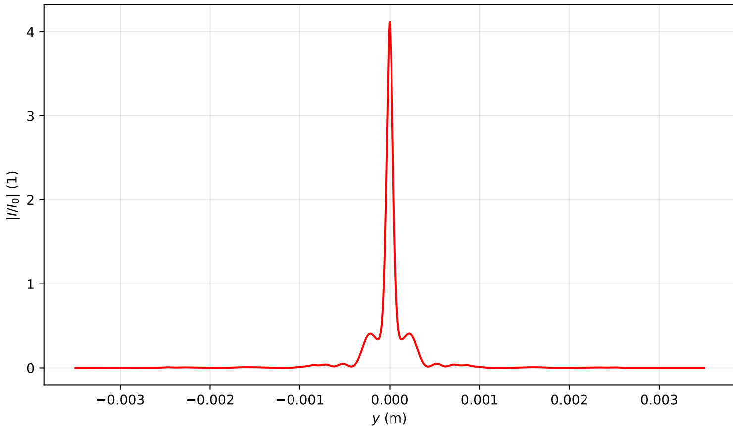
Intensity profile I(x = 0, y, z = 1.672)/I_0 , P_{in}=13.0P_{cr} , artificial time
